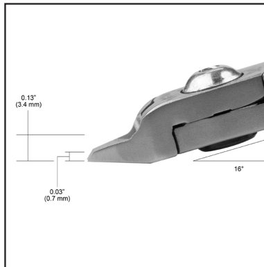
Relief Profile
