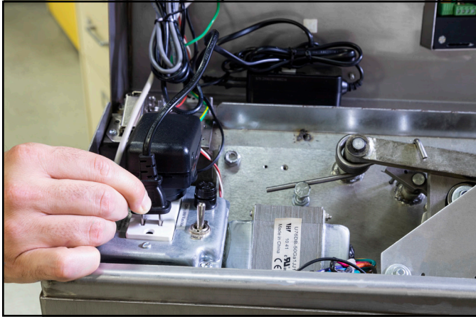
Figure 18. Connecting the power adapter to an electrical receptacle inside the turnstile
