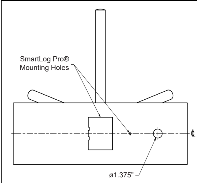
Figure 2. Mounting hole diameter for the Face Recognition Terminal's mounting post (inches)
