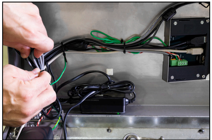
Figure 17. Organizing the cables
